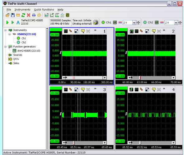
A 300 ms long USB signal, zoomed in at various factors. The lower right graph has a zoom factor of 30000. It still provides enough detail for accurate signal analysis.
